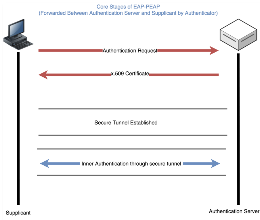
Figure 4 – The EAP-PEAP authentication process
