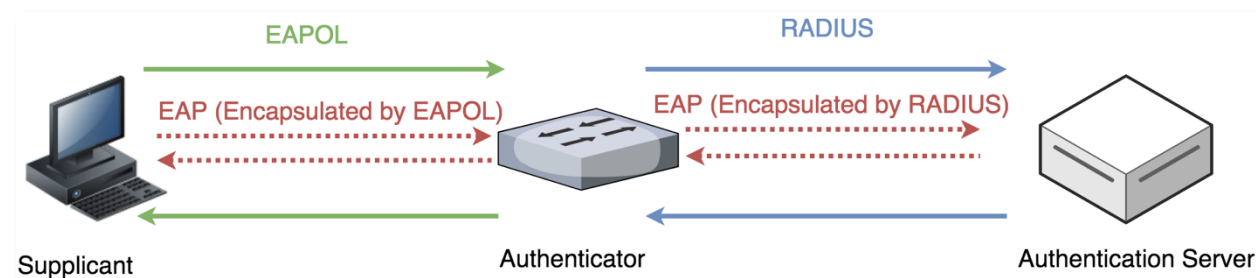
Figure 1 – The EAP authentication process is encapsulated by EAPOL between the supplicant and authenticator, and by RADIUS between the authenticator and authentication server.
