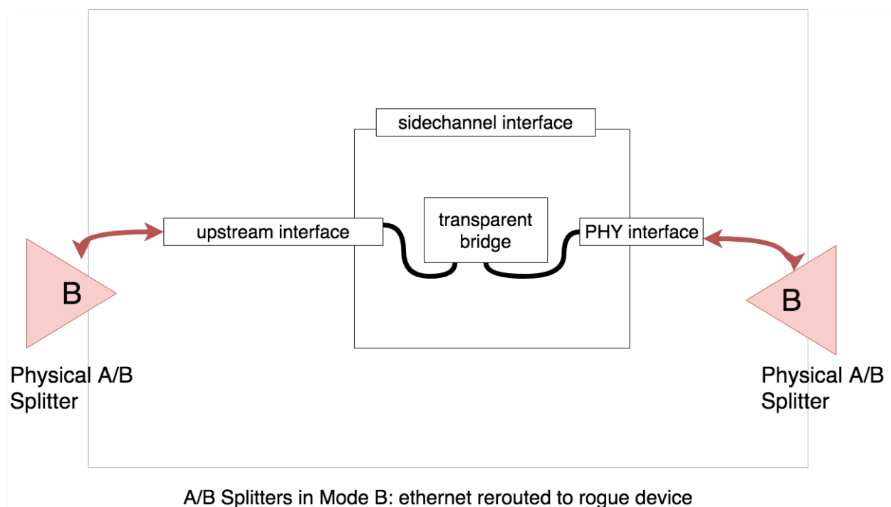
Figure 10 – Rogue Device B
