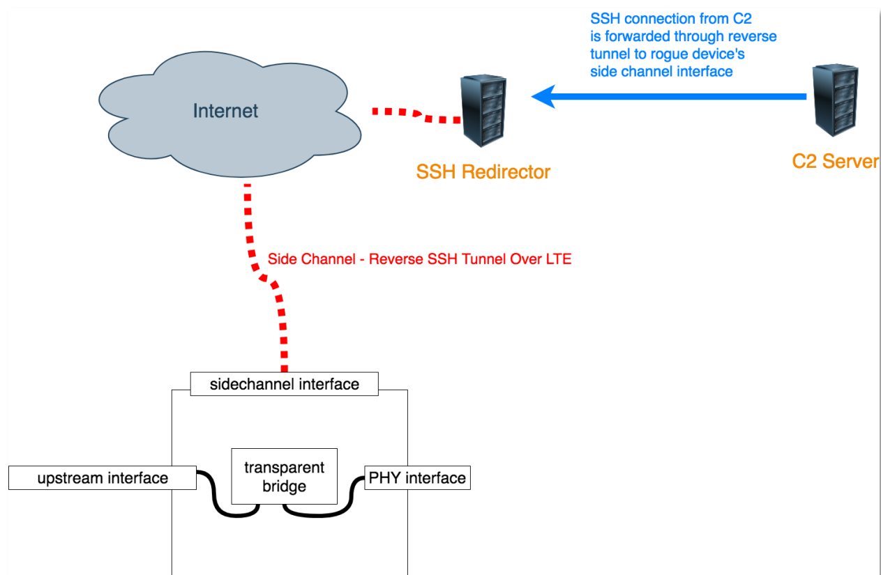
Figure 11 – Establishing a side channel using a reverse SSH tunnel over LTE
