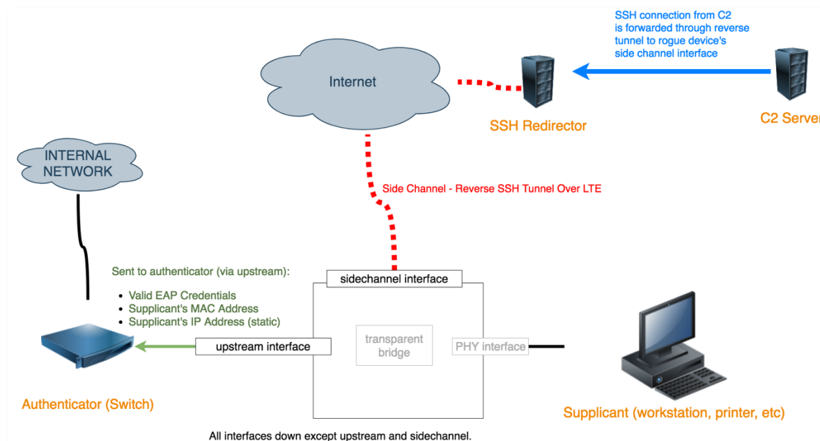
Figure 20 – performing a Bait n Switch attack
