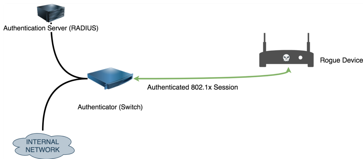
Figure 7 – objective: introducing a rogue device directly to the authenticator
