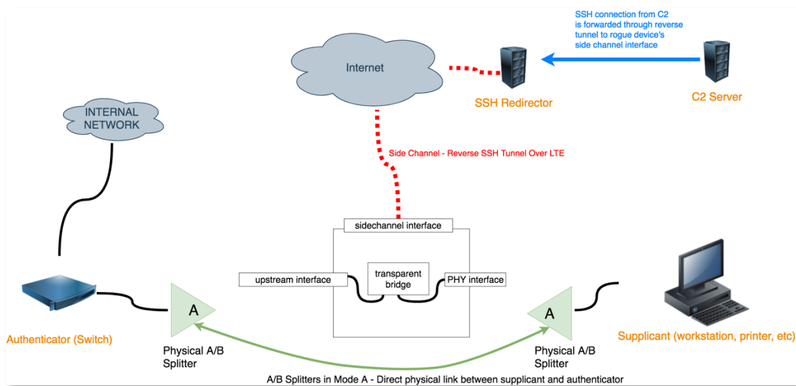
Figure 13 – the complete lab environment (using Rogue Device B)
