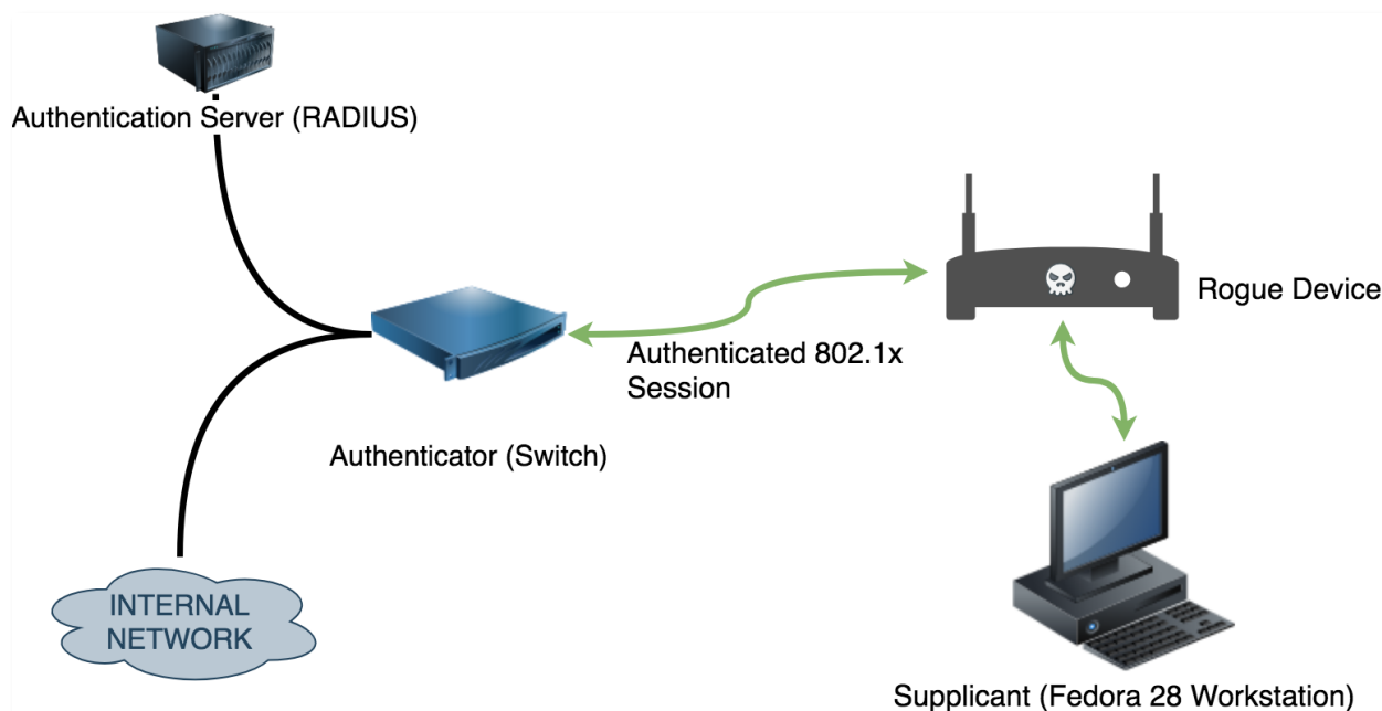
Figure 6 – objective: introducing a rogue device between the authenticator and supplicant
