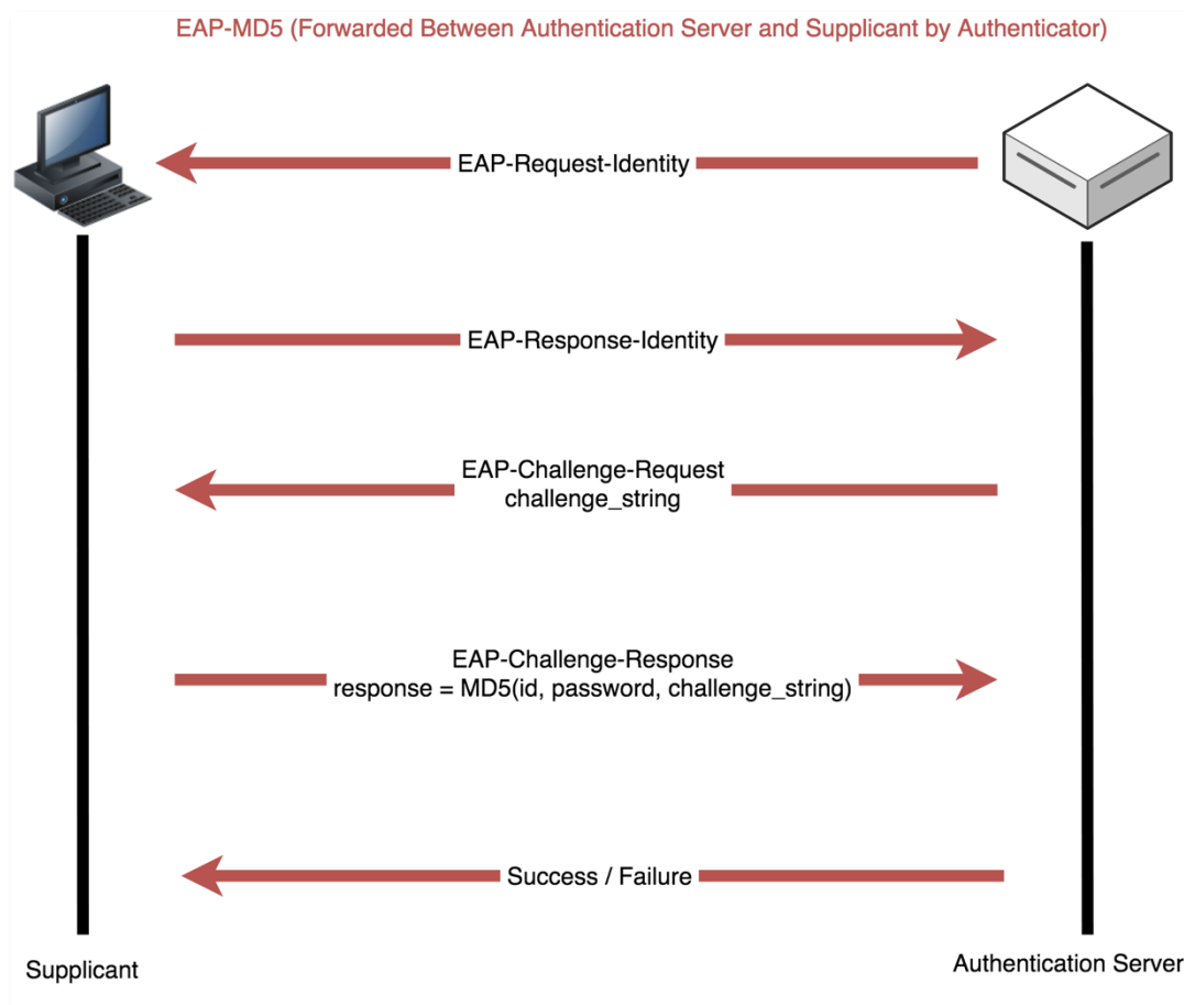
Figure 2 – the EAP-MD5 authentication process
