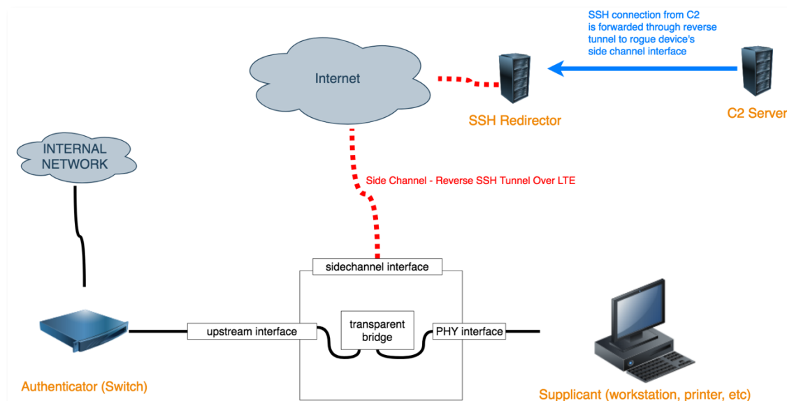
Figure 12 – the complete lab environment (using Rogue Device A)
